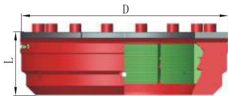
E-WE Type Casing Hanger
