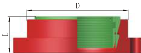
E-WD Type Casing Hanger
