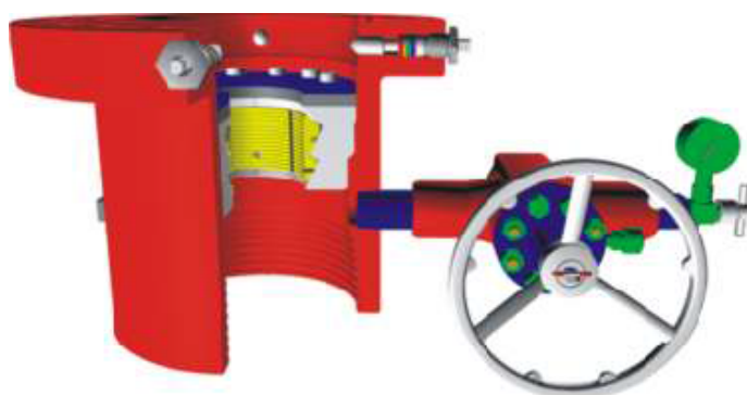
Threaded Bottom Connection Casing Head
